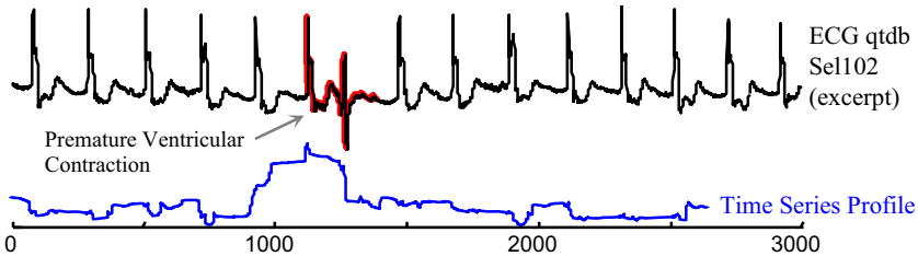
Fig. 19 (Top) An excerpt from an ECG incorporating a premature ventricular contraction ( red/bold ). (Bottom) The time series profile peaks exactly at the beginning of the PVC (Color figure online)
