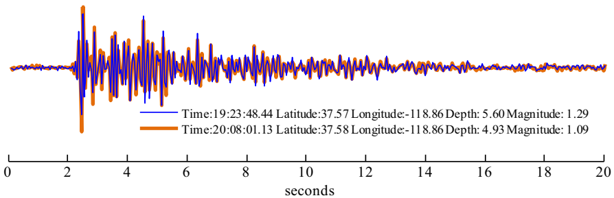
Fig. 9 A set of doublets extracts from the seismic data recorded at a station near Mammoth Lakes on February 17th, 2016. One occurrence ( fine/blue ) is overlaid on top of another occurrence ( bold/orange ) that happened about 45 min later (Color figure online)
